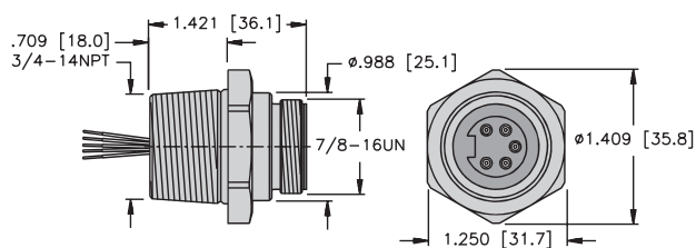
"A" P-RSF .. 14.75/NPT
