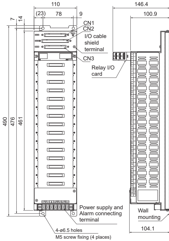
DC Power Supply (RVV-31)
