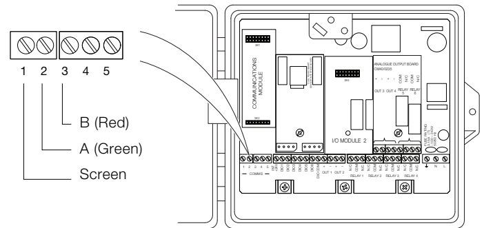
Fig. 4.2 Aztec AWT440 PCB connections to Profibus network
